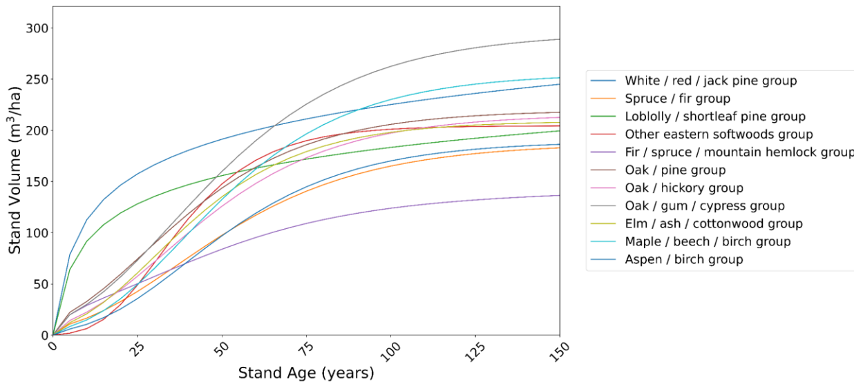
Figure S1. Example of empirically derived yield curves for forest type groups in Maryland with full stocking (ALSTKCD=2).
