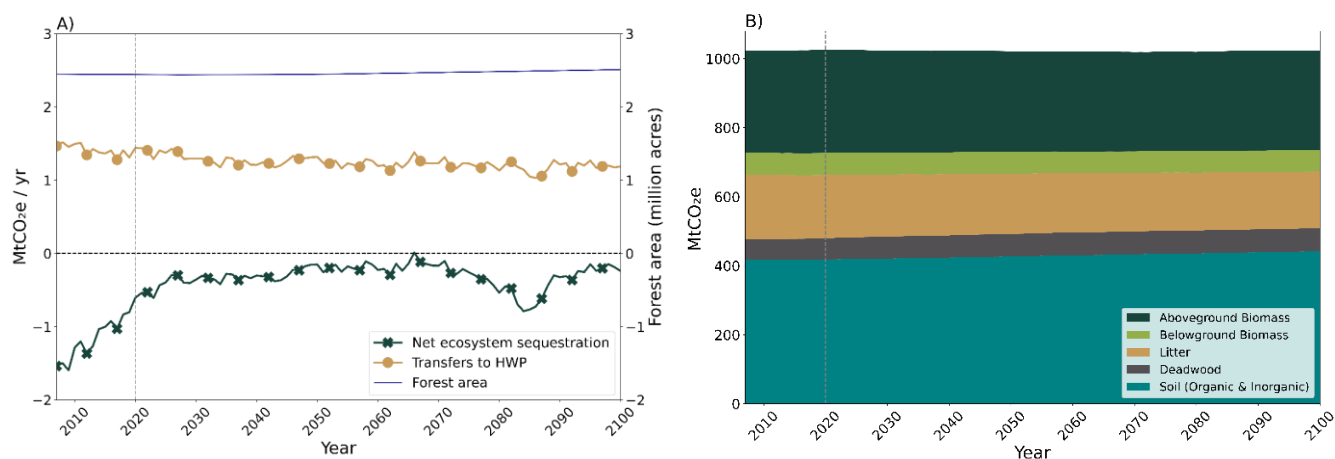
Figure 4. BAU scenario results showing A) annual net ecosystem sequestration and transfers to HWP (both in MtCO 2e /yr), forest area (million acres) and B) carbon stocks (MtCO 2e ) in IPCC reporting pools from 2007–2100. Net ecosystem sequestration refers to the net yearly sequestration of carbon by forests after accounting for decomposition and wood product removals. Negative numbers for net ecosystem sequestration in Panel A) represent a net carbon sink, and positive numbers for transfers to HWP in Panel A) and positive numbers in Panel B) represent accruing carbon stocks.
