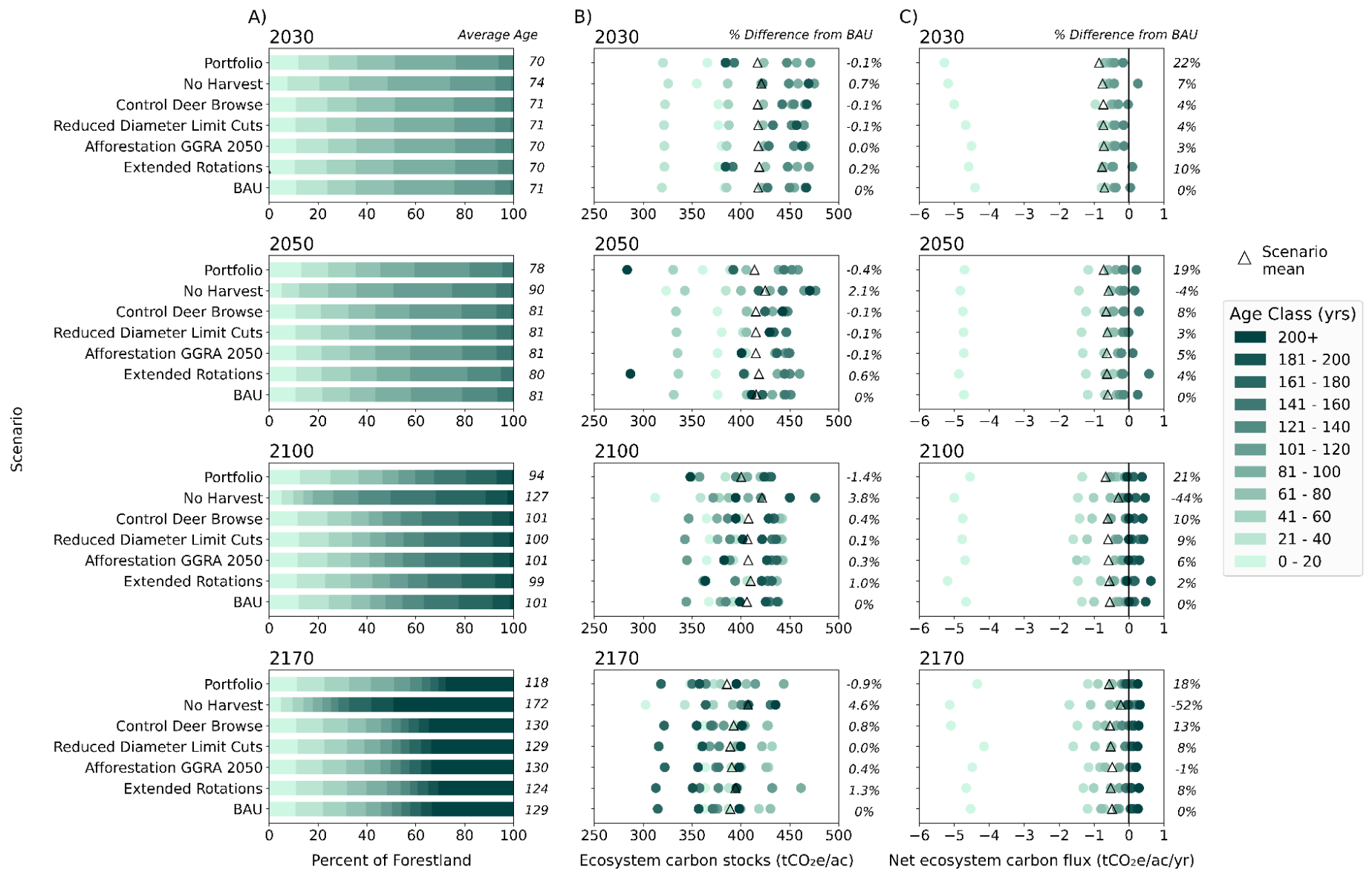
Figure 11. A) Age class distribution, B) carbon stock density ( tCO_2e/ac ), and C) carbon flux density ( tCO_2e/ac/yr ) for selected scenarios in 2030, 2050, 2100, and 2170. In Panel B), positive values denote accruing carbon stocks. In Panel C), negative values denote carbon sequestration and positive values denote carbon emissions.
