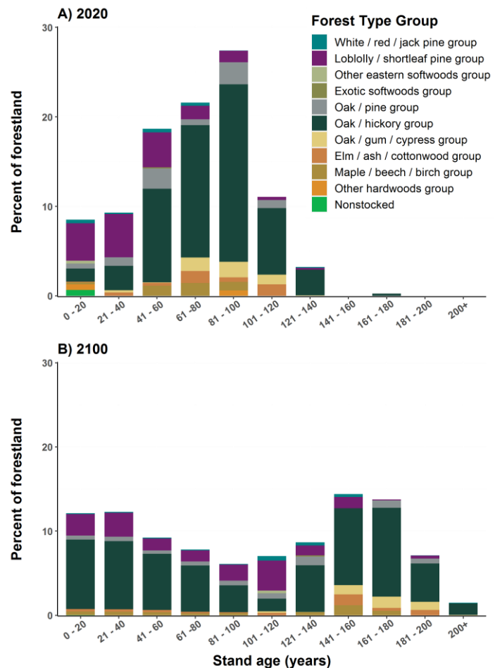
Figure 6. BAU scenario age class distribution by forest type group in A) 2020 and B) 2100.
